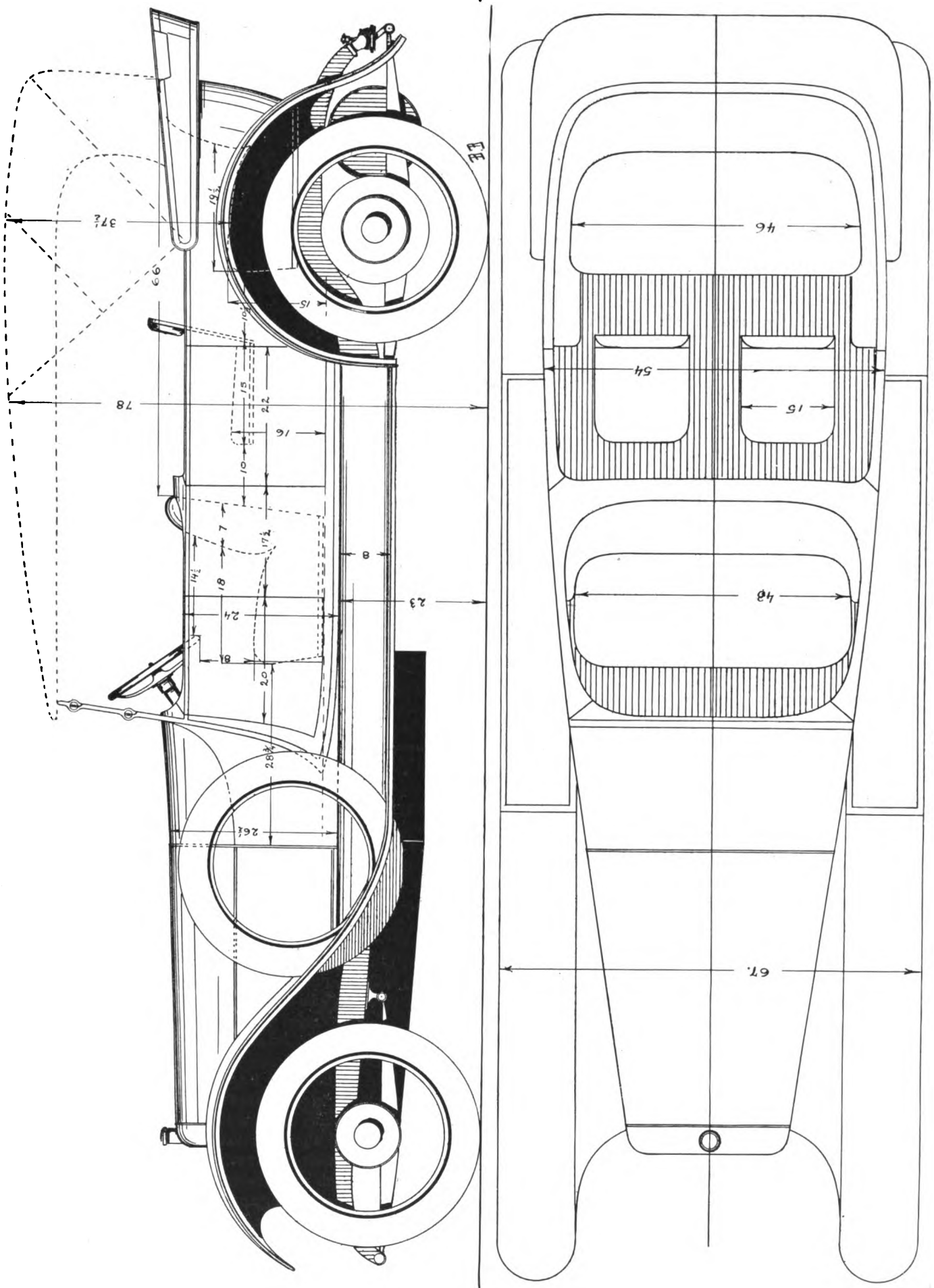
SEVEN-PASSENGER TOURING BODY Description on opposite page
